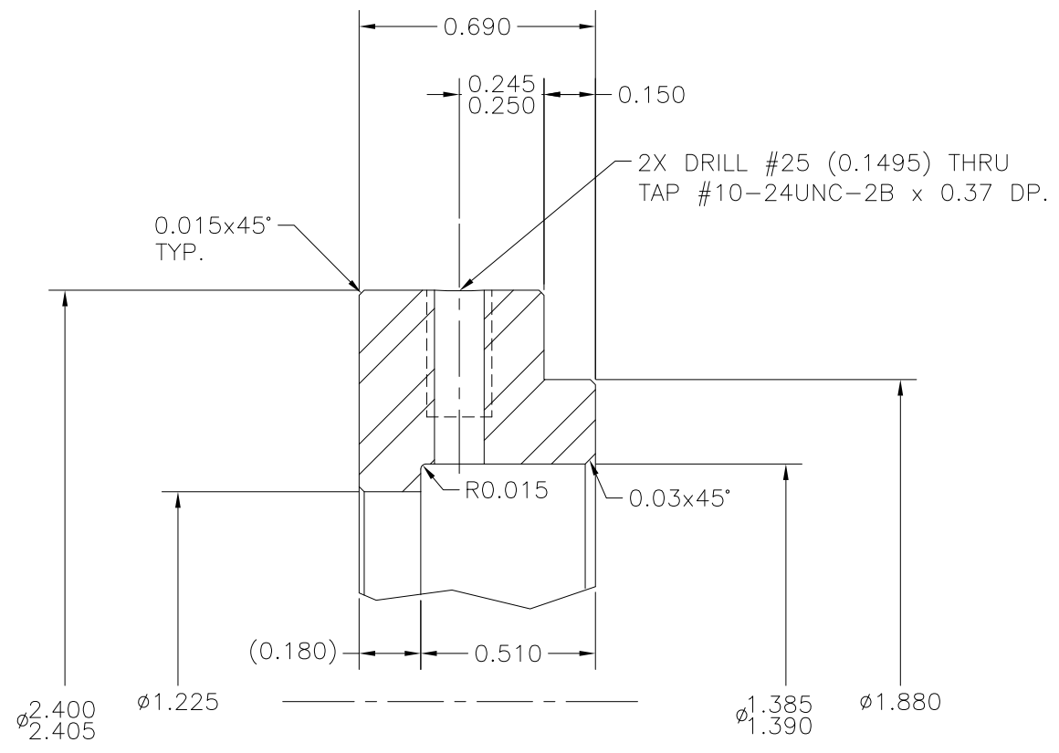
SECTION 1-C-3 REF. 1-B-6
