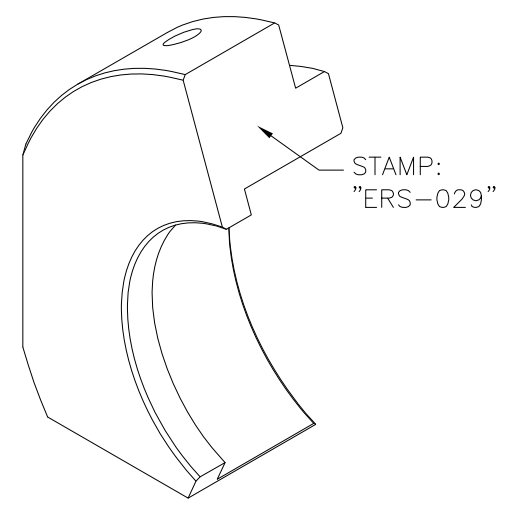
PICTORIAL 1-B-3 UPPER BEARING HOLDER N.T.S.
