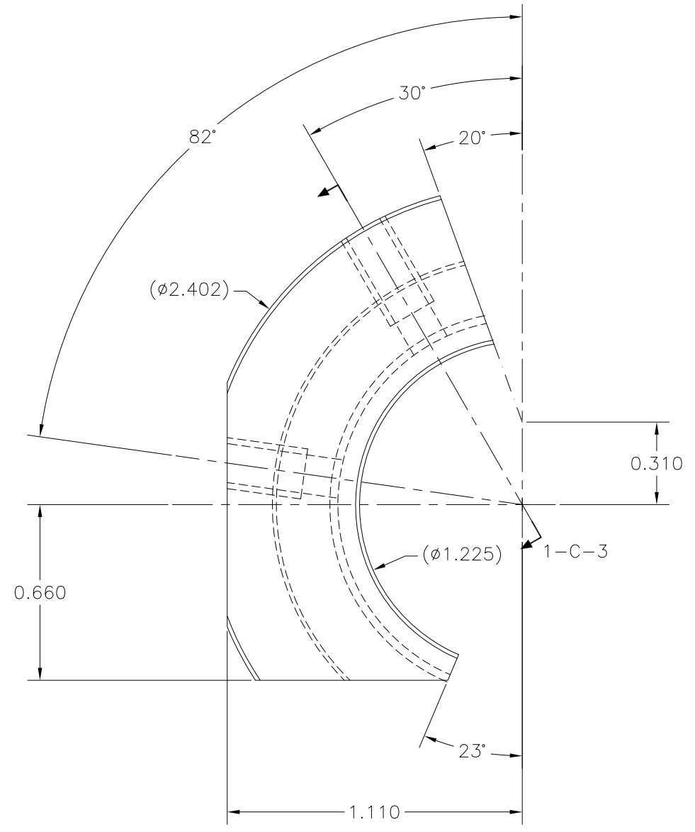
END VIEW 1-C-7 UPPER BEARING HOLDER ONE REQ'D AS SHOWN ONE REQ'D MIRROR IMAGE
